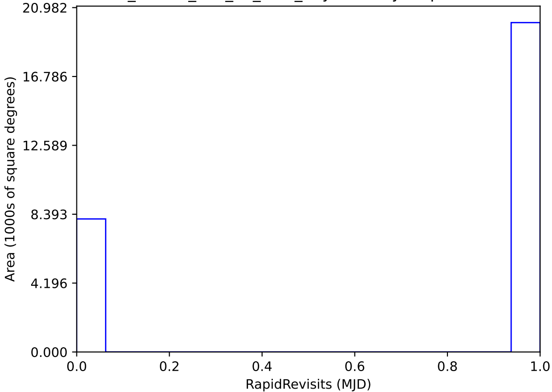
ddf_loaded_half_fl2_v3.4_10yrs All sky: RapidRevisits
