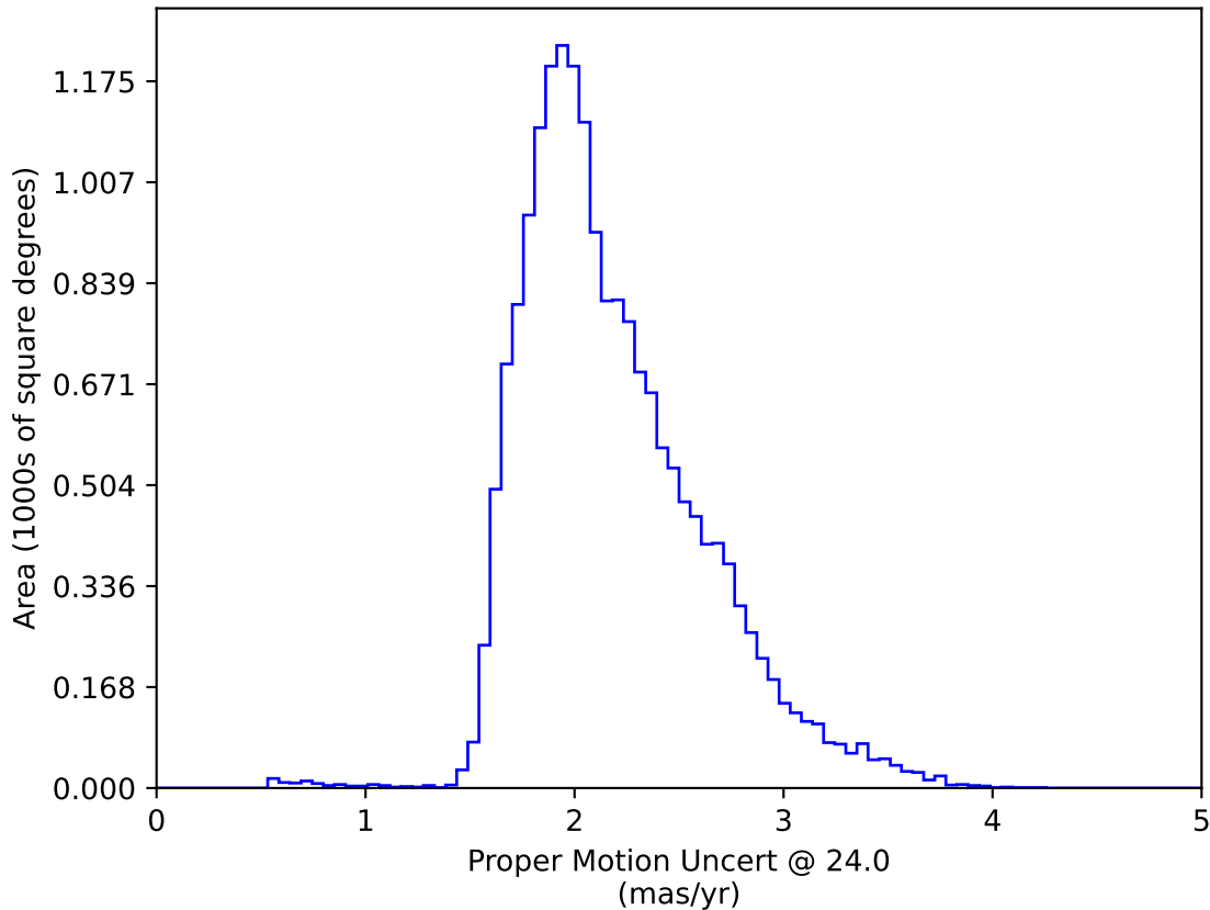
ddf_loaded_half_fl2_v3.4_10yrs WFD: Proper Motion Uncert @ 24.0
