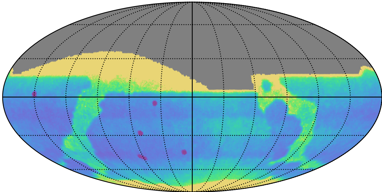
ddf_loaded_half_fl2_v3.4_10yrs All sky: Proper Motion Uncert @ 24.0
