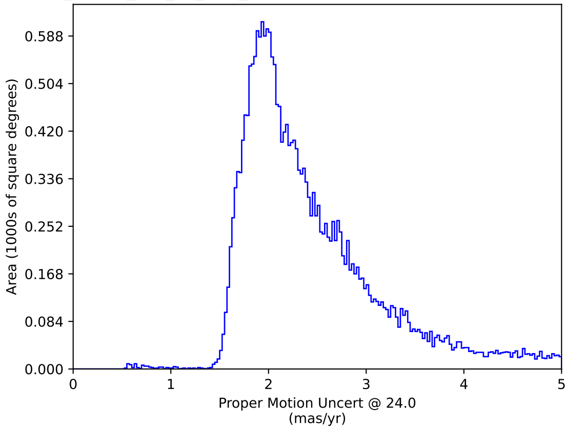
ddf_loaded_half_fl2_v3.4_10yrs All sky: Proper Motion Uncert @ 24.0
