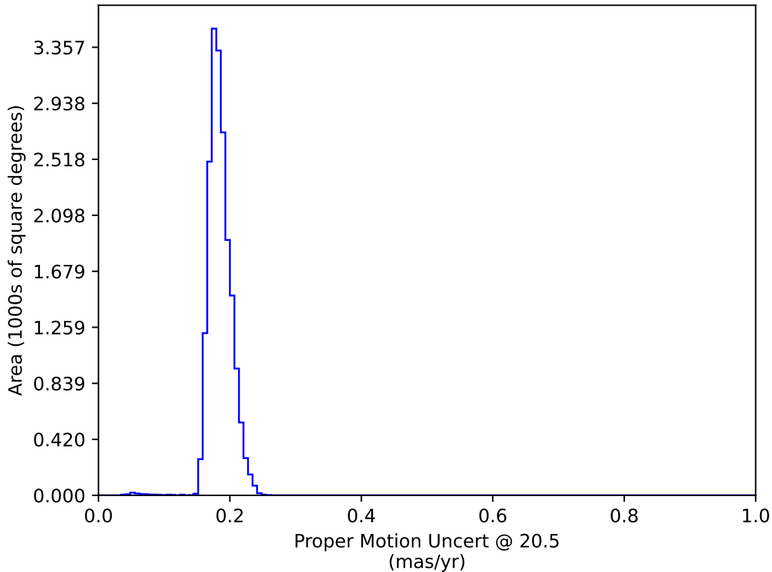
ddf_loaded_half_fl2_v3.4_10yrs WFD: Proper Motion Uncert @ 20.5
