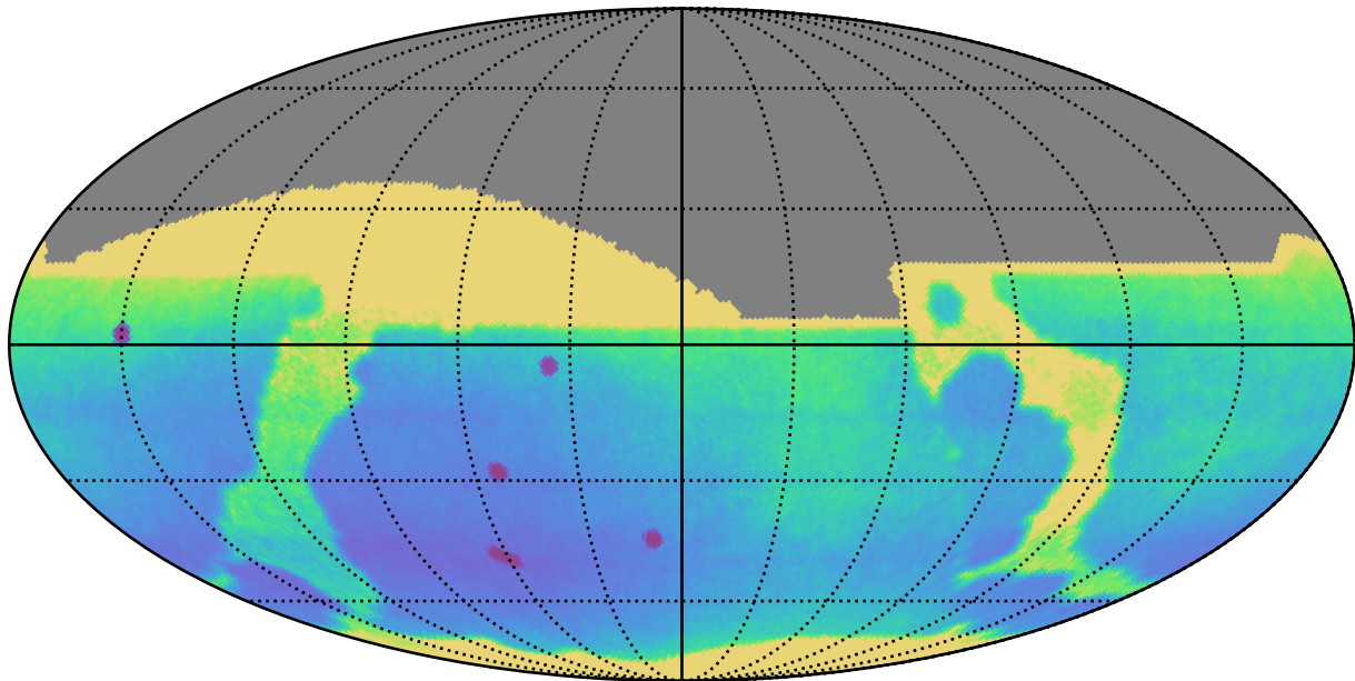
ddf_loaded_half_fl2_v3.4_10yrs All sky: Parallax Uncert @ 24.0
