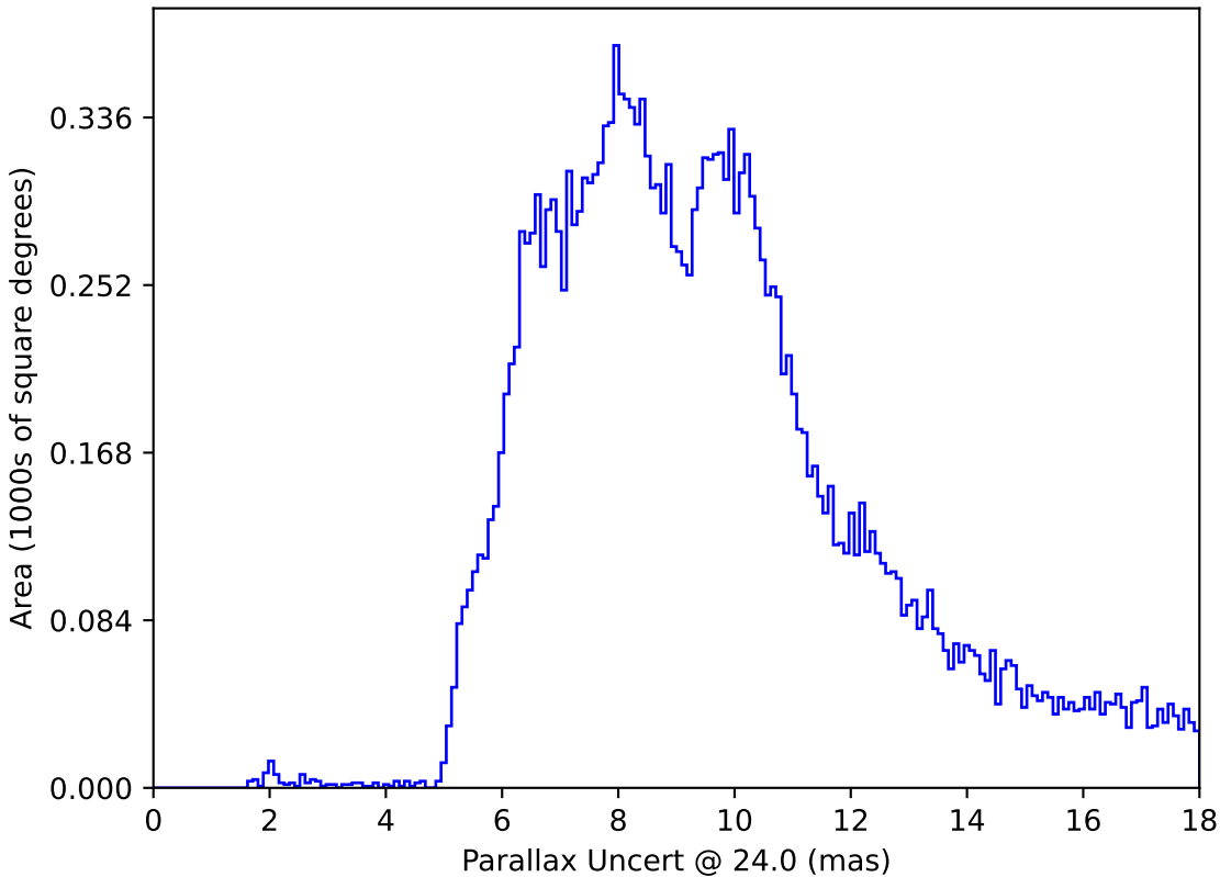
ddf_loaded_half_fl2_v3.4_10yrs All sky: Parallax Uncert @ 24.0
