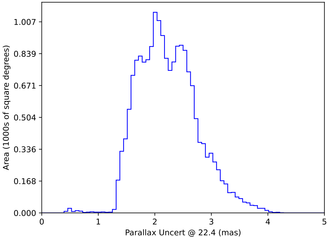
ddf_loaded_half_fl2_v3.4_10yrs WFD: Parallax Uncert @ 22.4
