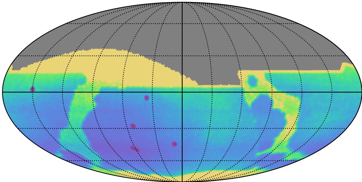
ddf_loaded_half_fl2_v3.4_10yrs All sky: Parallax Uncert @ 22.4
