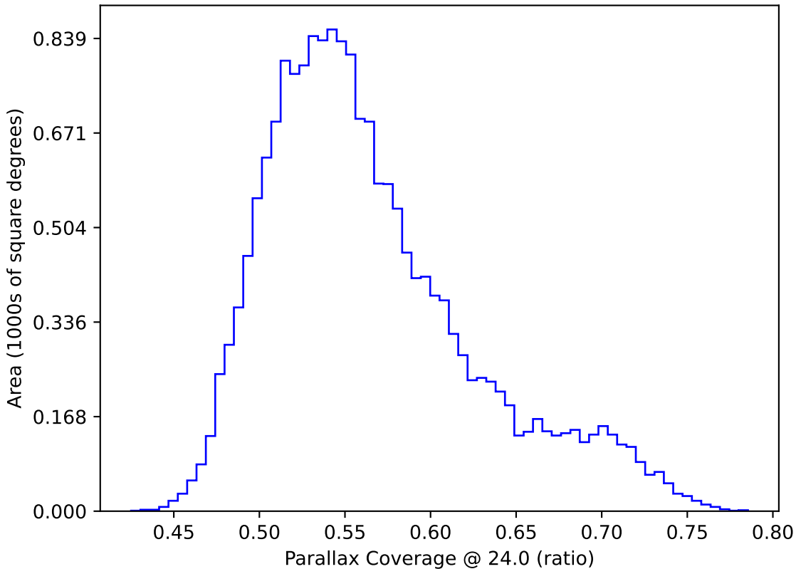
ddf_loaded_half_fl2_v3.4_10yrs WFD: Parallax Coverage @ 24.0
