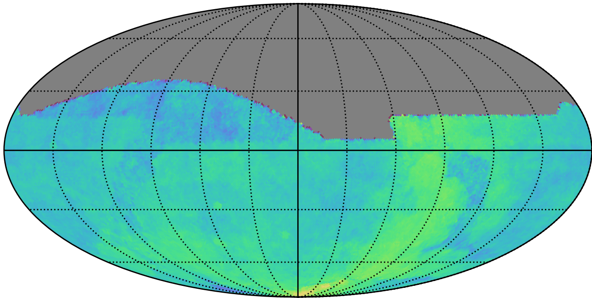
ddf_loaded_half_fl2_v3.4_10yrs All sky: Parallax Coverage @ 24.0
