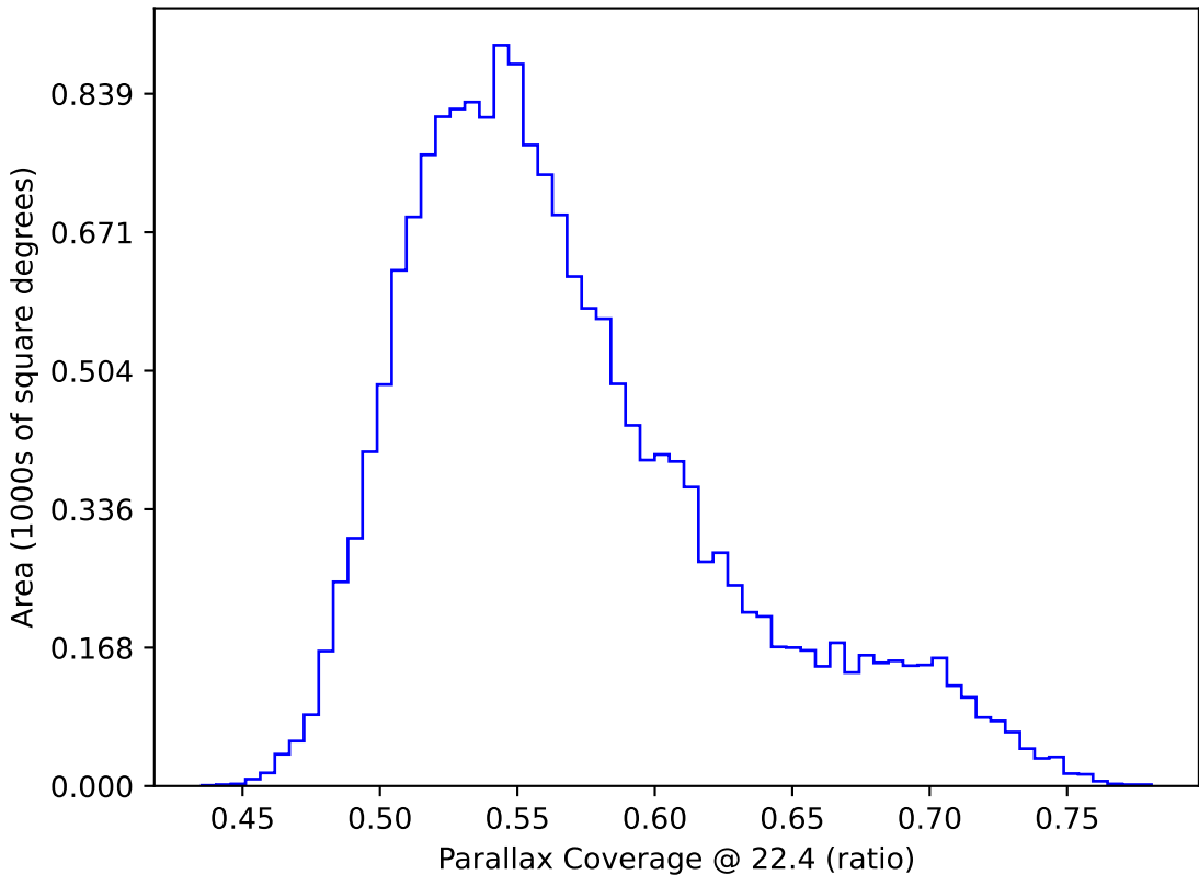
ddf_loaded_half_fl2_v3.4_10yrs WFD: Parallax Coverage @ 22.4
