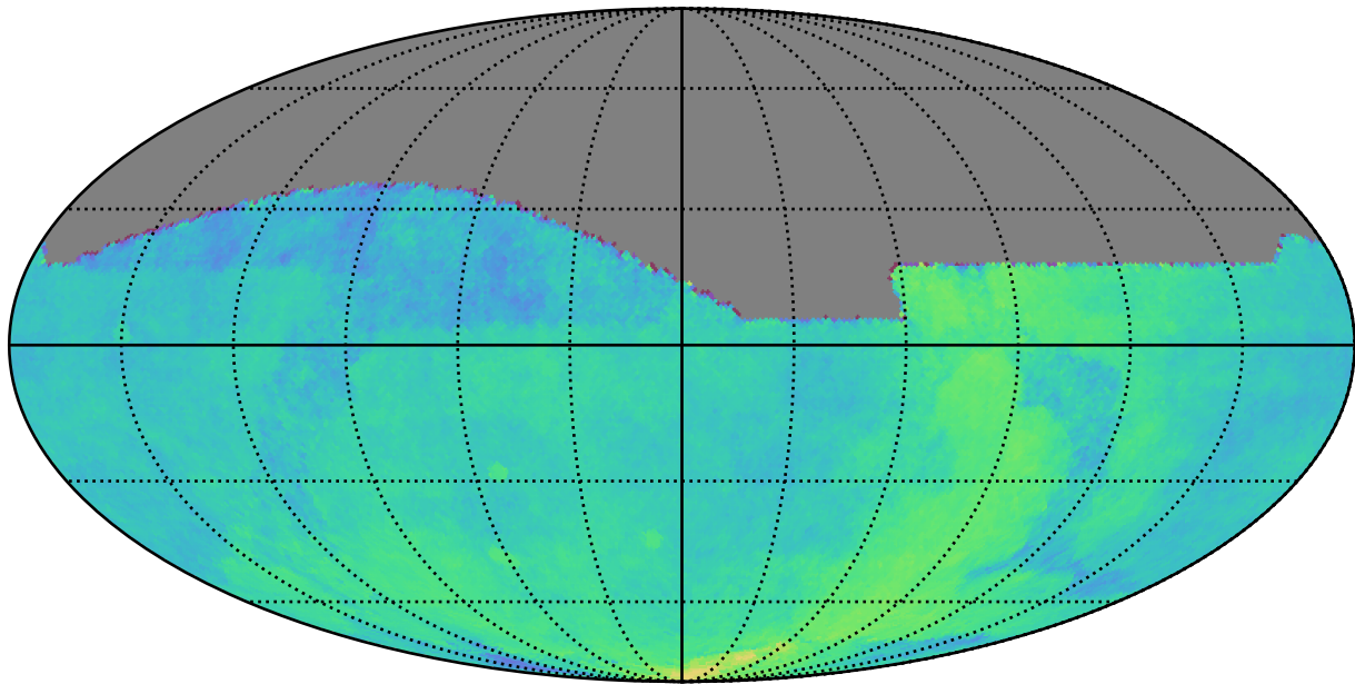
ddf_loaded_half_fl2_v3.4_10yrs All sky: Parallax Coverage @ 22.4
