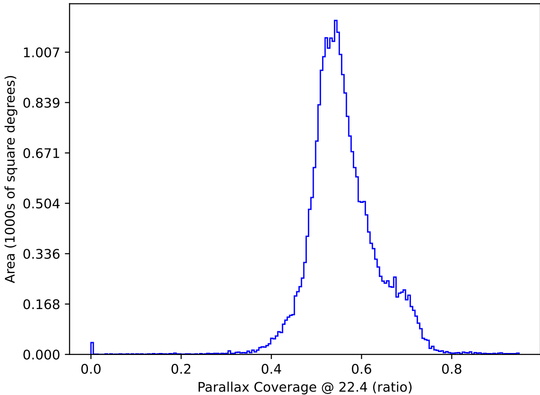
ddf_loaded_half_fl2_v3.4_10yrs All sky: Parallax Coverage @ 22.4
