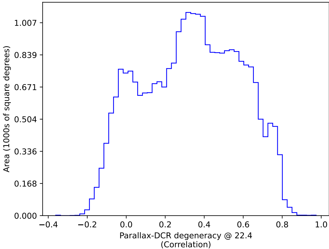
ddf_loaded_half_fl2_v3.4_10yrs All sky: Parallax-DCR degeneracy @ 22.4
