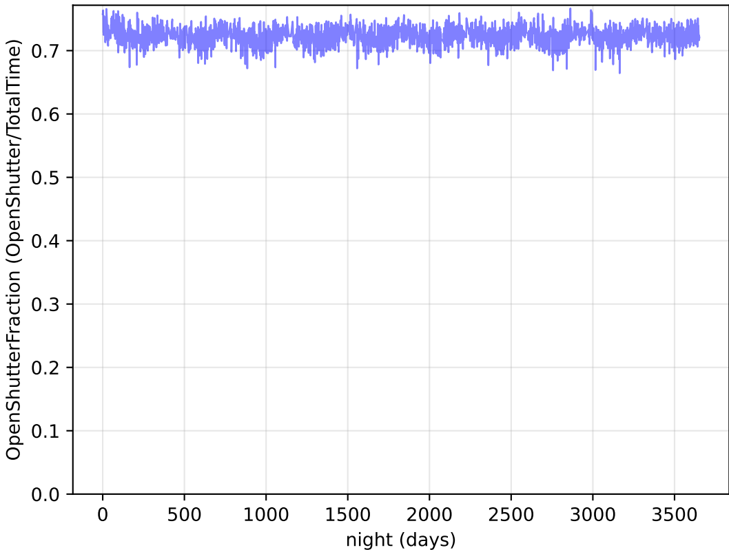
ddf_loaded_half_fl2_v3.4_10yrs Per night: OpenShutterFraction
