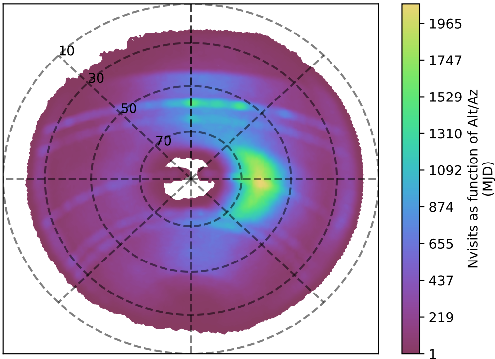
ddf_loaded_half_fl2_v3.4_10yrs z band: Nvisits as function of Alt/Az
