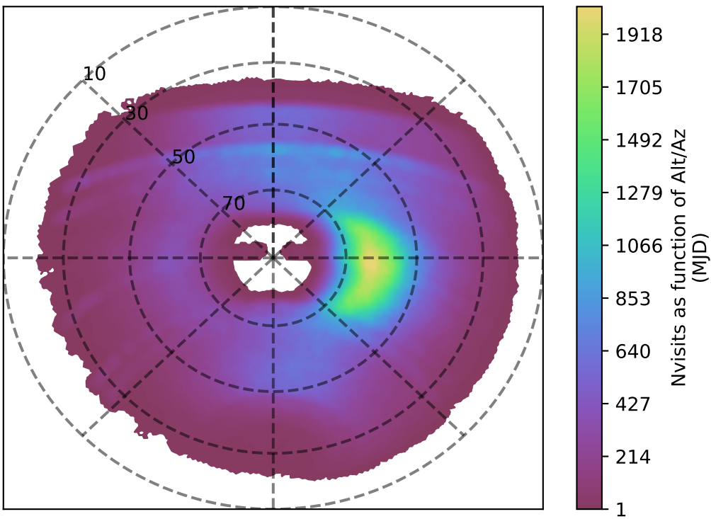
ddf_loaded_half_fl2_v3.4_10yrs y band: Nvisits as function of Alt/Az
