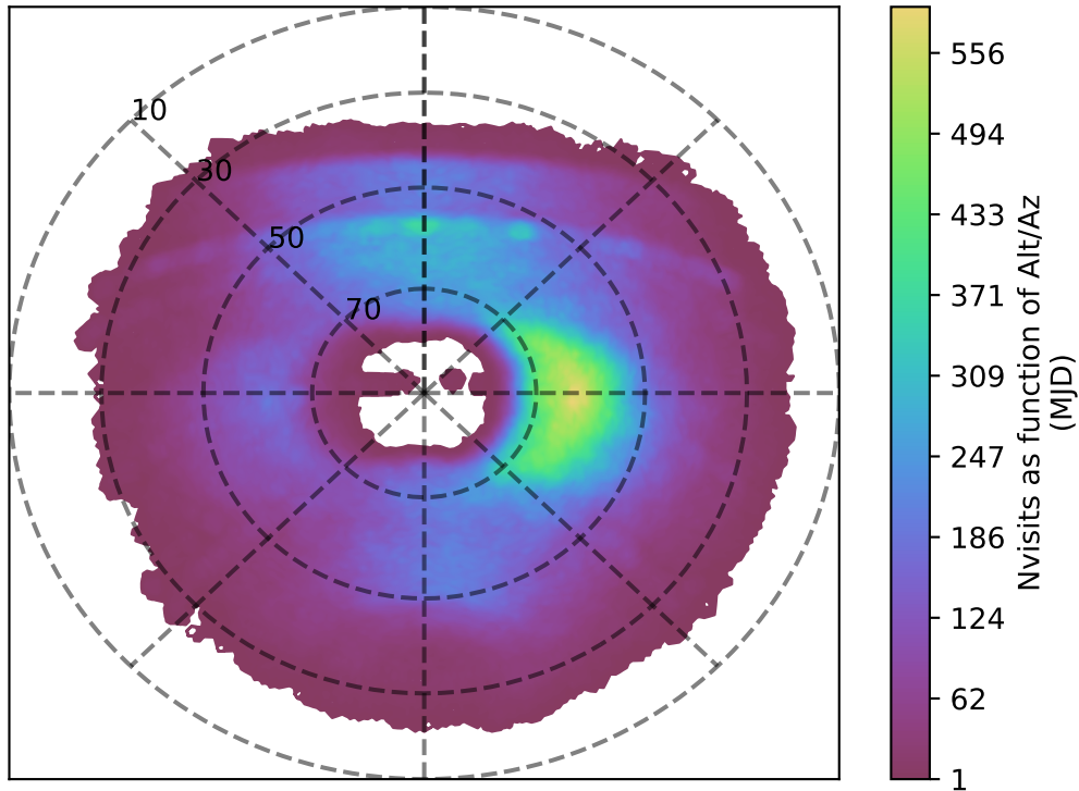
ddf_loaded_half_fl2_v3.4_10yrs u band: Nvisits as function of Alt/Az
