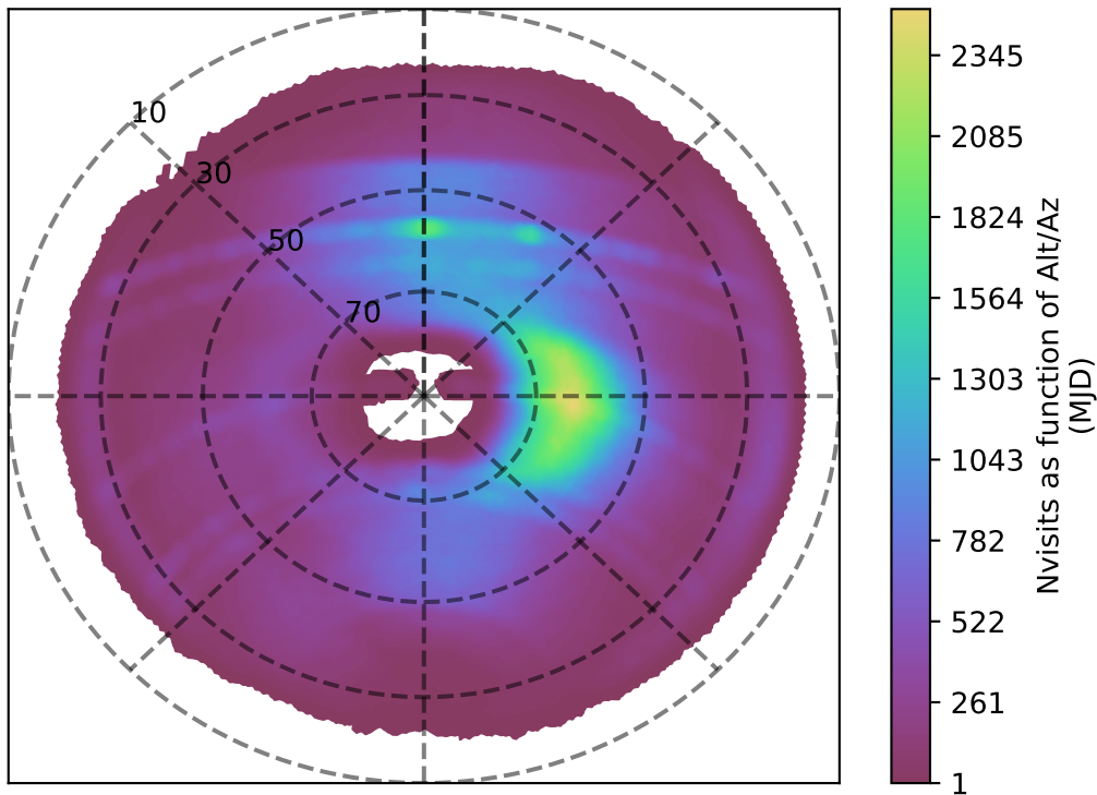
ddf_loaded_half_fl2_v3.4_10yrs i band: Nvisits as function of Alt/Az
