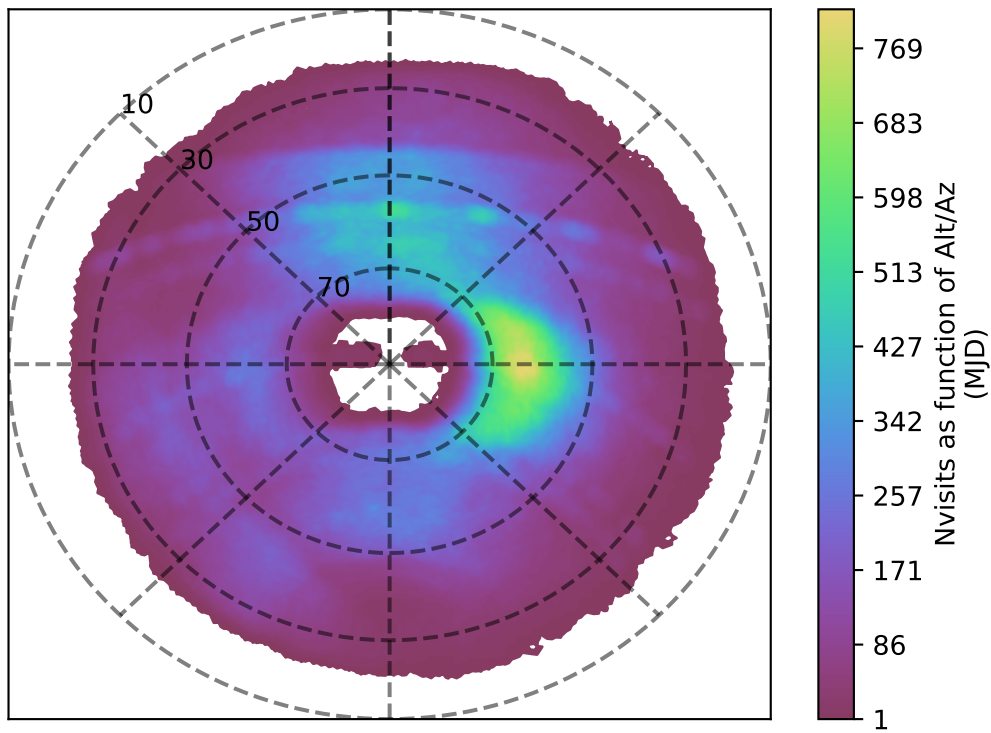
ddf_loaded_half_fl2_v3.4_10yrs g band: Nvisits as function of Alt/Az
