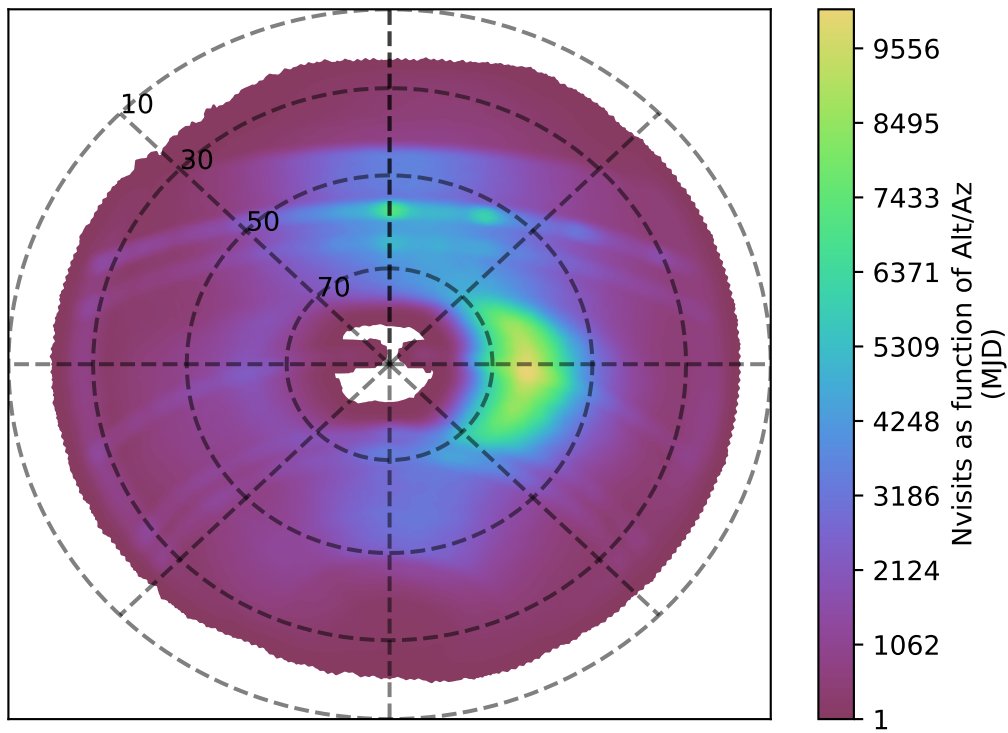
ddf_loaded_half_f12_v3.4_10yrs all bands: Nvisits as function of Alt/Az
