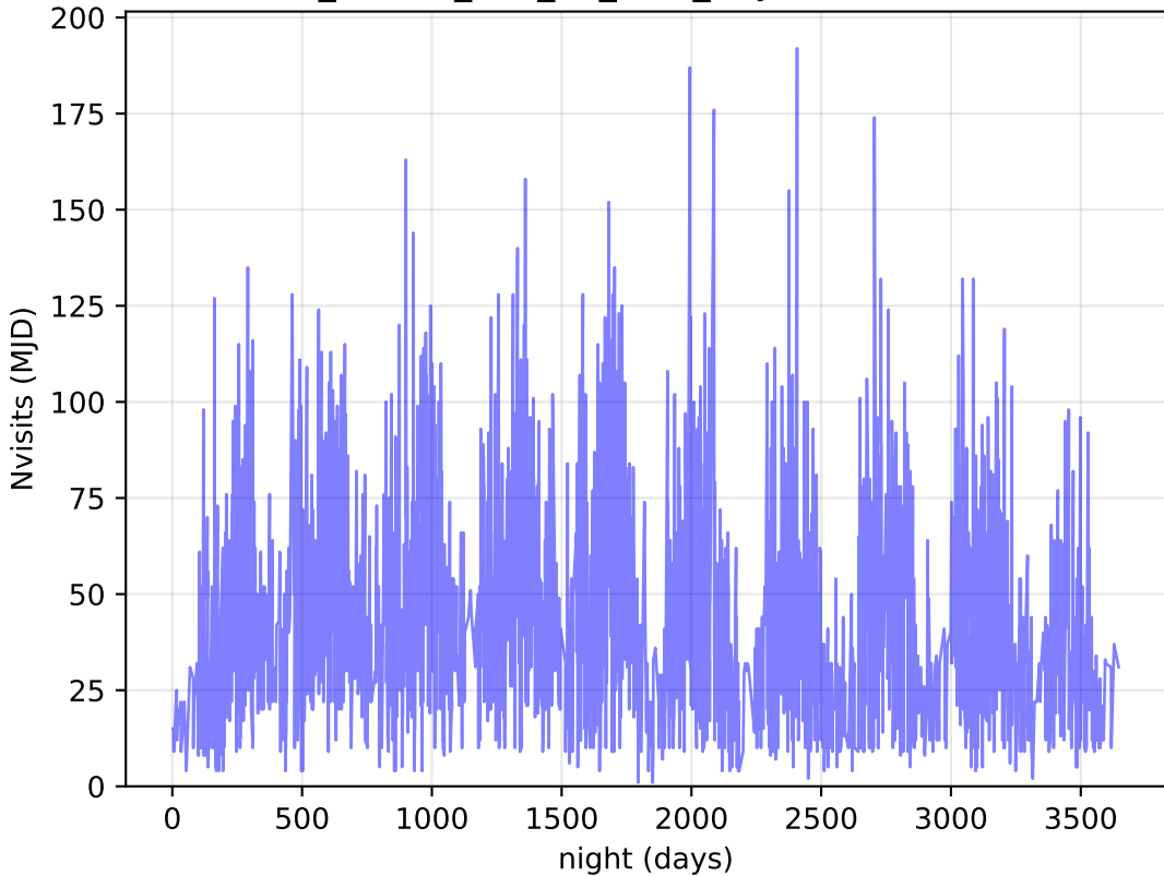
ddf_loaded_half_fl2_v3.4_10yrs DDF: Nvisits
