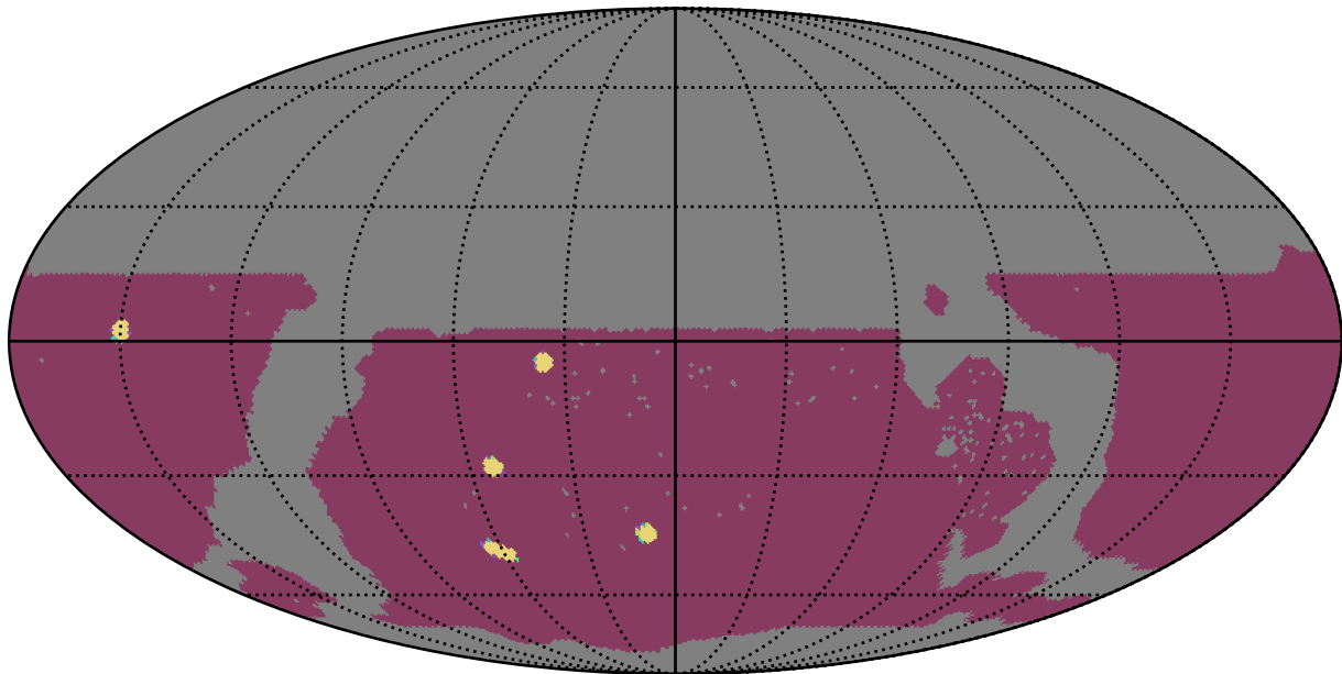
ddf_loaded_half_fl2_v3.4_10yrs WFD: NumberOfQuickRevisits
