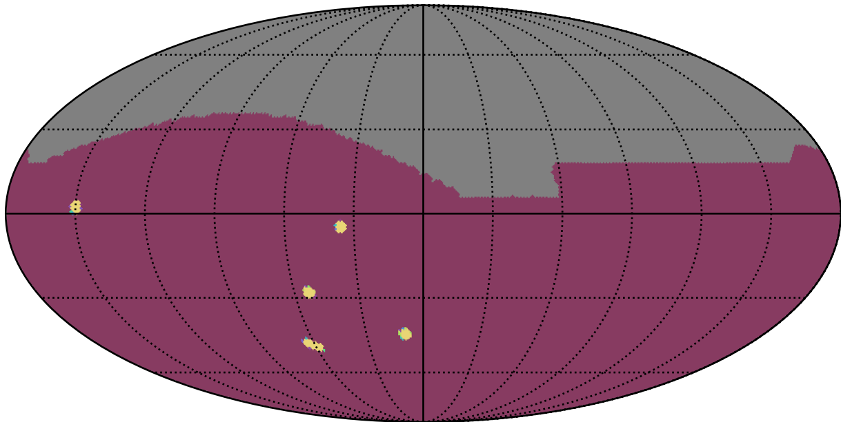
ddf_loaded_half_fl2_v3.4_10yrs All sky: NumberOfQuickRevisits
