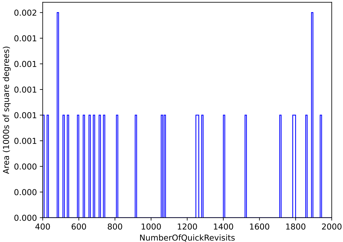
ddf_loaded_half_fi2_v3.4_10yrs All sky: NumberOfQuickRevisits
