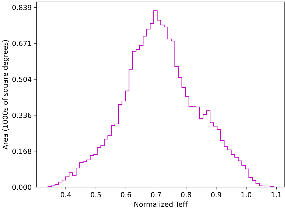
ddf_loaded_half_fl2_v3.4_10yrs WFD z band: Normalized Teff
