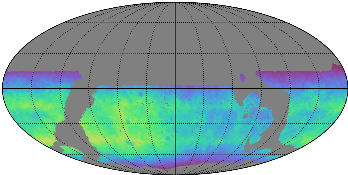
ddf_loaded_half_fl2_v3.4_10yrs WFD y band: Normalized Teff
