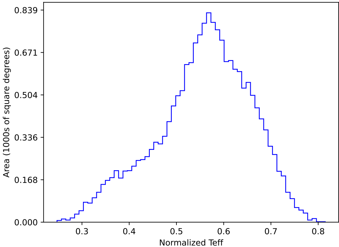
ddf_loaded_half_fl2_v3.4_10yrs WFD y band: Normalized Teff
