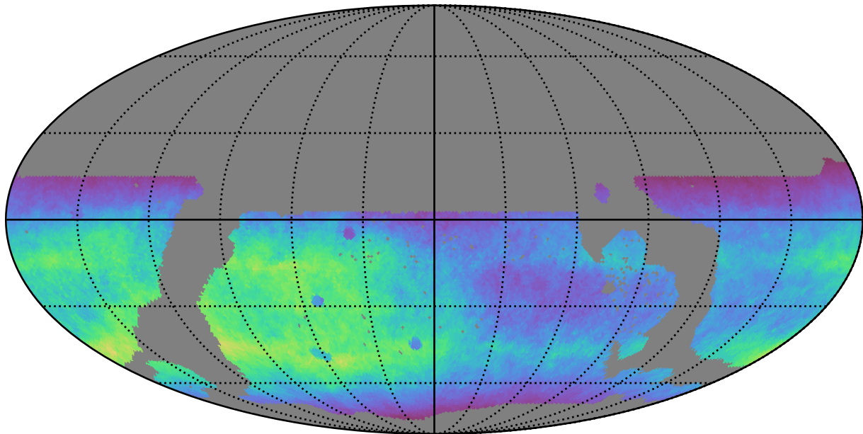
ddf_loaded_half_fl2_v3.4_10yrs WFD r band: Normalized Teff
