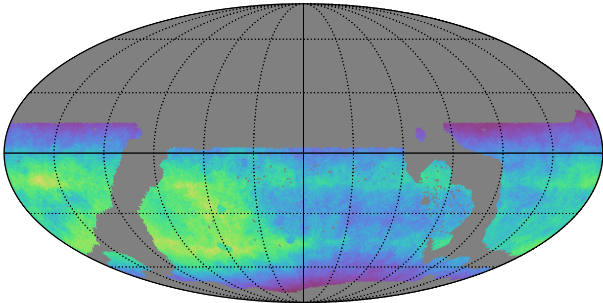
ddf_loaded_half_fl2_v3.4_10yrs WFD i band: Normalized Teff
