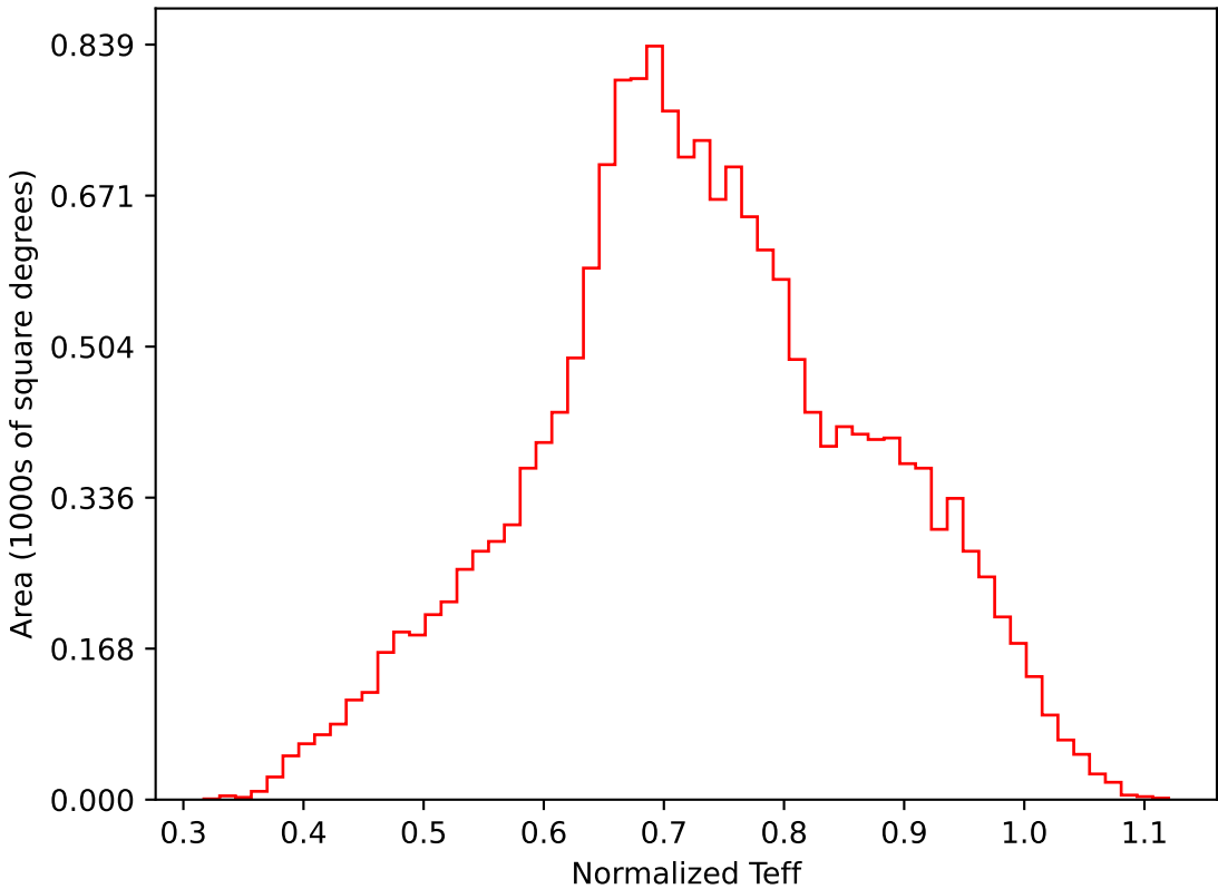
ddf_loaded_half_fl2_v3.4_10yrs WFD i band: Normalized Teff
