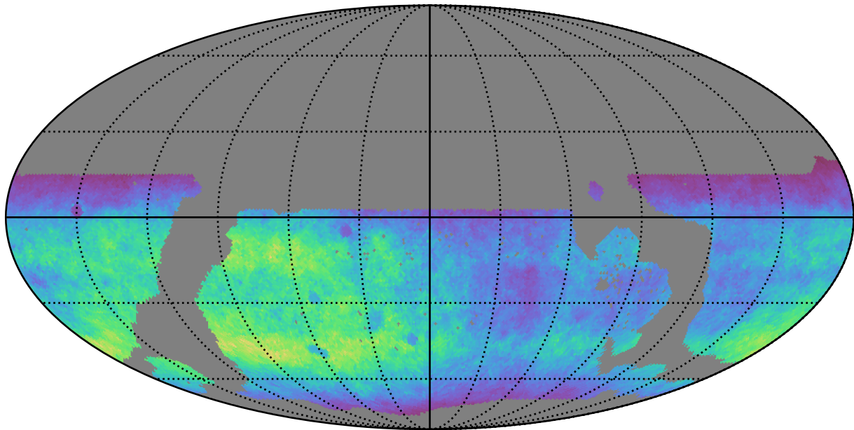
ddf_loaded_half_fl2_v3.4_10yrs WFD g band: Normalized Teff
