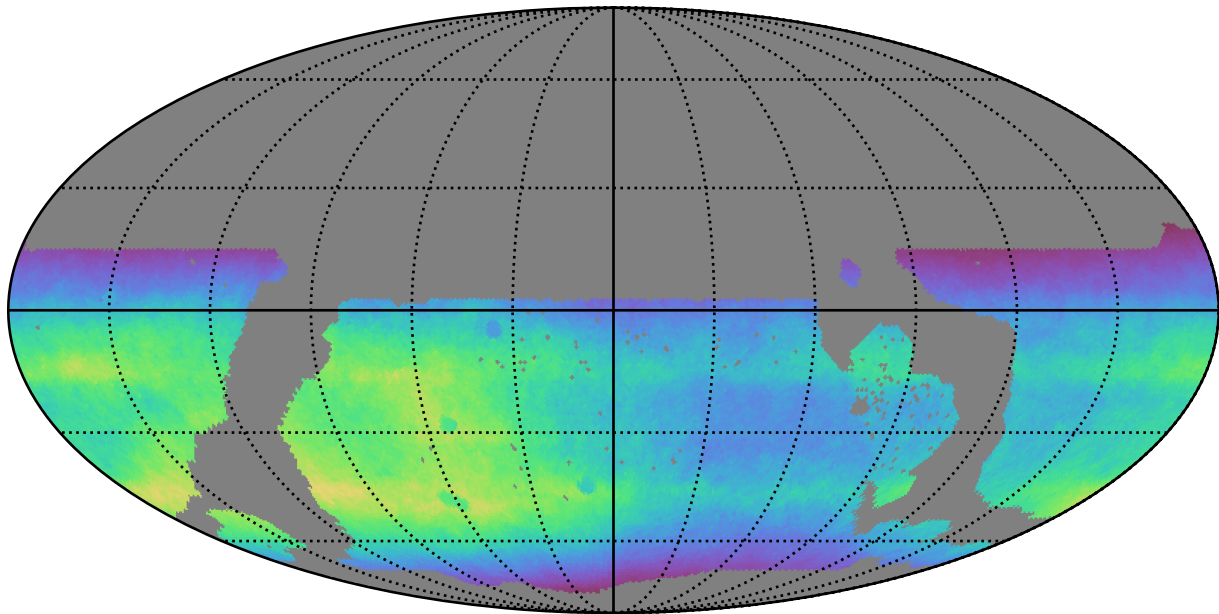
ddf_loaded_half_fl2_v3.4_10yrs WFD all bands: Normalized Teff
