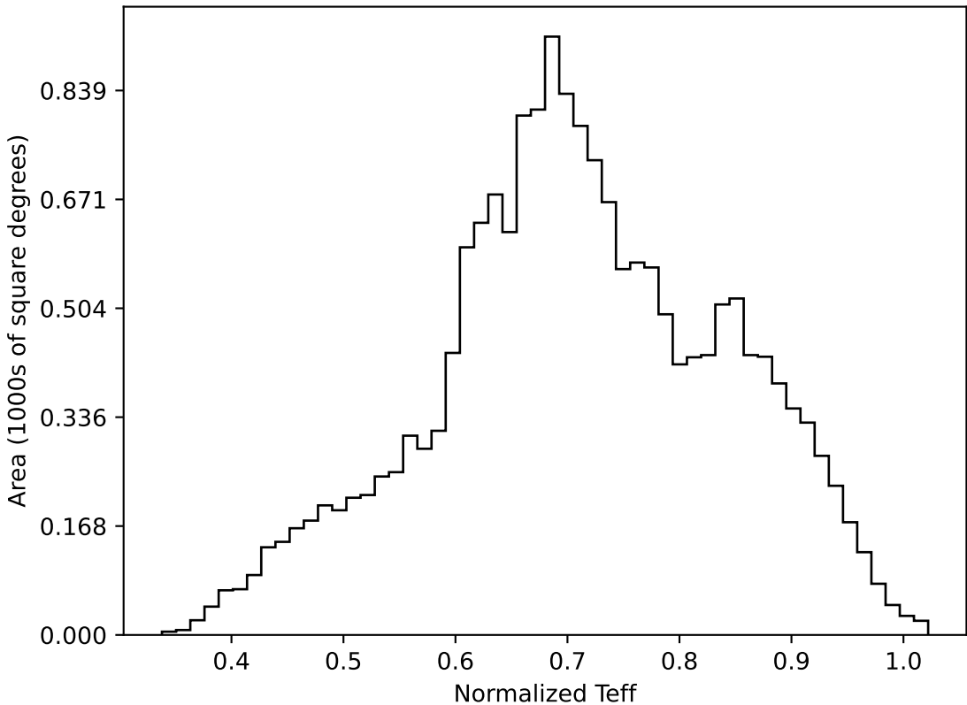
ddf_loaded_half_fl2_v3.4_10yrs WFD all bands: Normalized Teff
