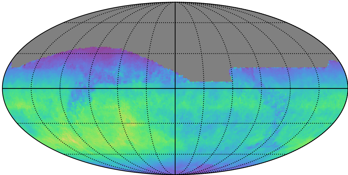
ddf_loaded_half_fl2_v3.4_10yrs All sky z band: Normalized Teff
