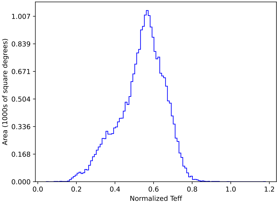
ddf_loaded_half_fl2_v3.4_10yrs All sky y band: Normalized Teff
