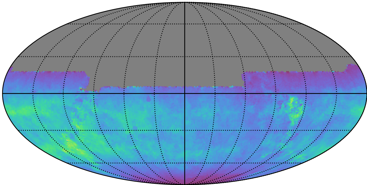
ddf_loaded_half_fl2_v3.4_10yrs All sky u band: Normalized Teff
