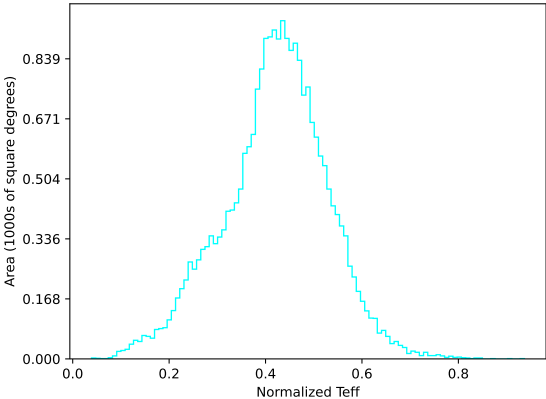
ddf_loaded_half_fl2_v3.4_10yrs All sky u band: Normalized Teff
