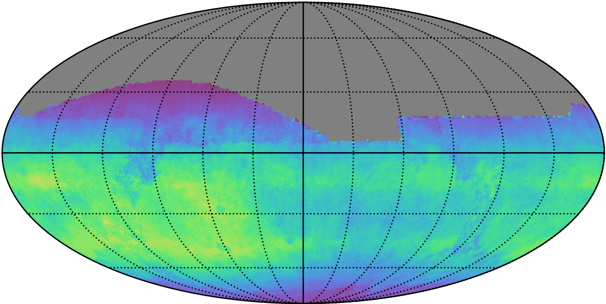
ddf_loaded_half_fl2_v3.4_10yrs All sky i band: Normalized Teff
