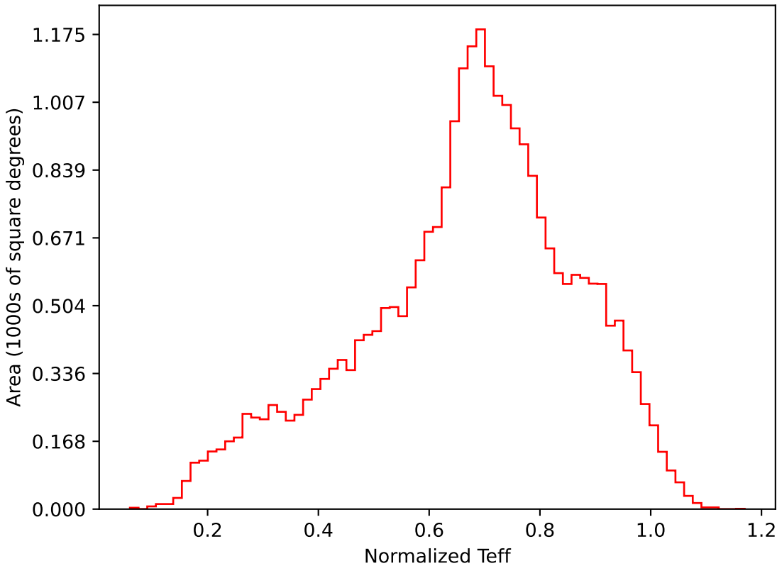
ddf_loaded_half_fl2_v3.4_10yrs All sky i band: Normalized Teff
