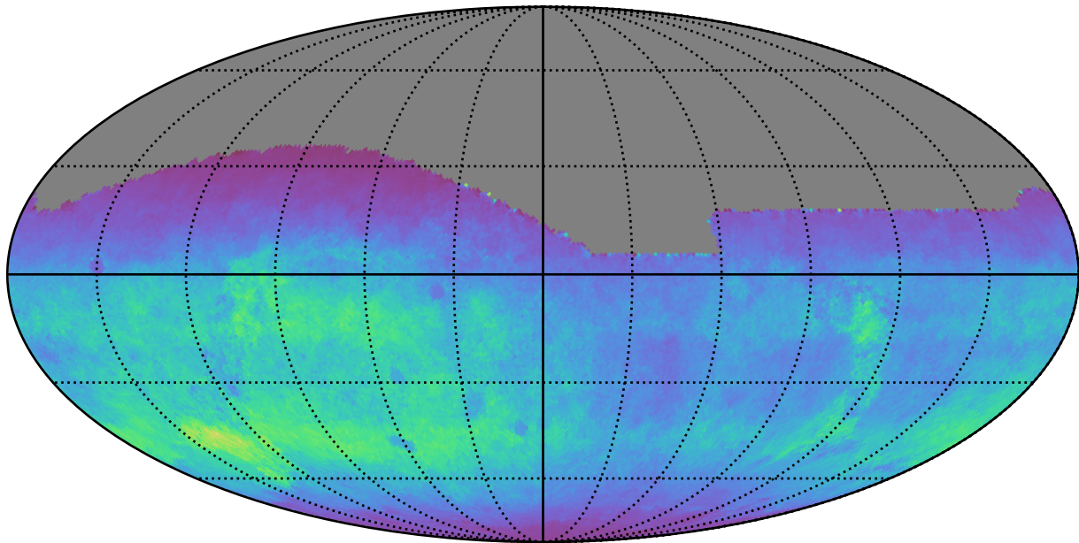
ddf_loaded_half_fl2_v3.4_10yrs All sky g band: Normalized Teff
