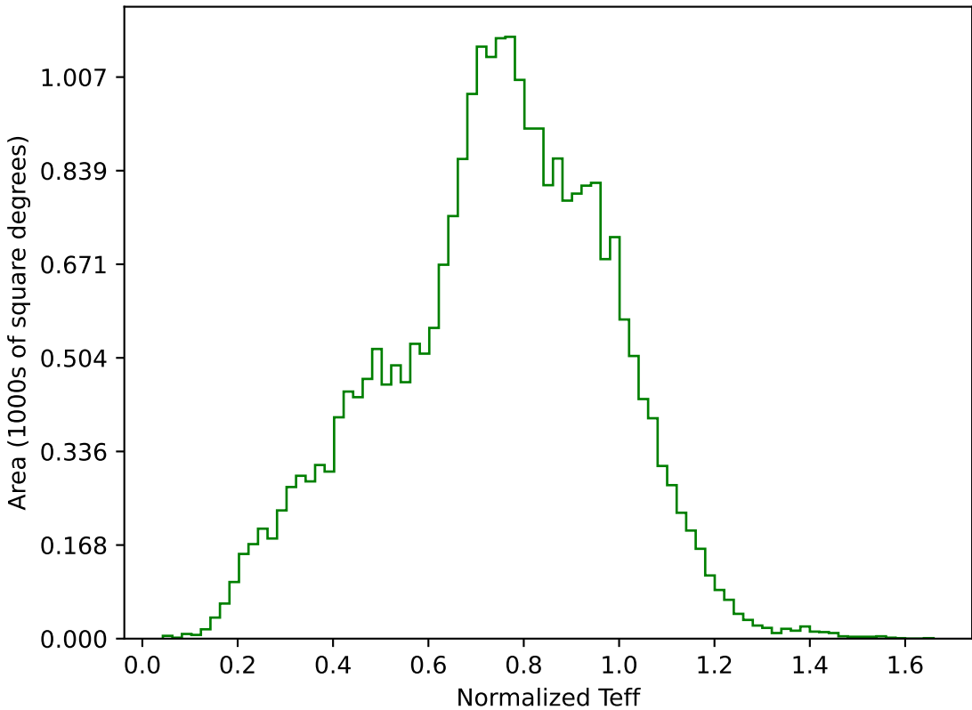
ddf_loaded_half_fl2_v3.4_10yrs All sky g band: Normalized Teff
