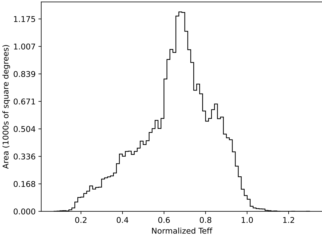
ddf_loaded_half_fl2_v3.4_10yrs All sky all bands: Normalized Teff
