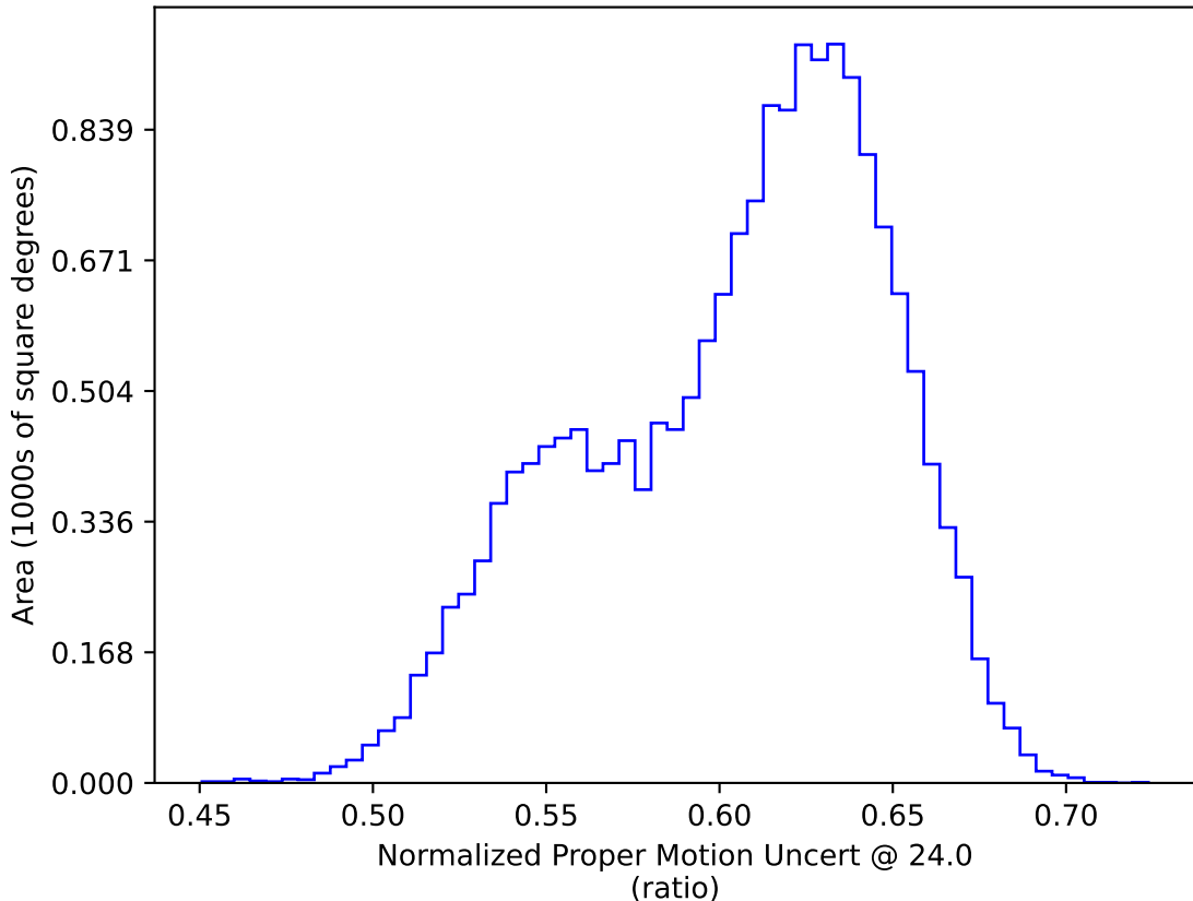
ddf_loaded_half_fl2_v3.4_10yrs WFD: Normalized Proper Motion Uncert @ 24.0
