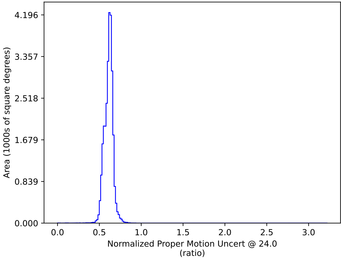
ddf_loaded_half_fl2_v3.4_10yrs All sky: Normalized Proper Motion Uncert @ 24.0
