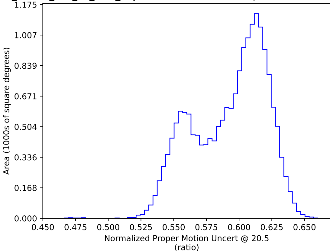
ddf_loaded_half_fl2_v3.4_10yrs WFD: Normalized Proper Motion Uncert @ 20.5
