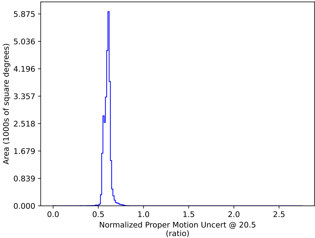
ddf_loaded_half_fl2_v3.4_10yrs All sky: Normalized Proper Motion Uncert @ 20.5
