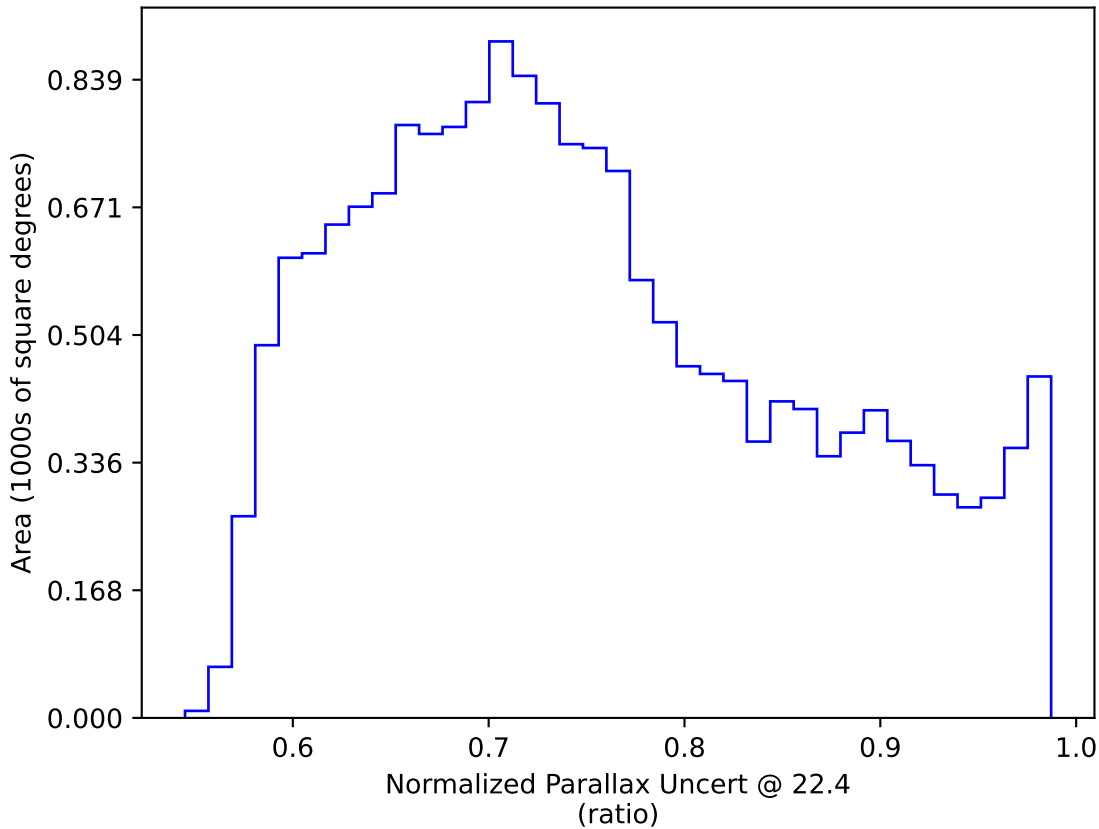
ddf_loaded_half_fl2_v3.4_10yrs WFD: Normalized Parallax Uncert @ 22.4
