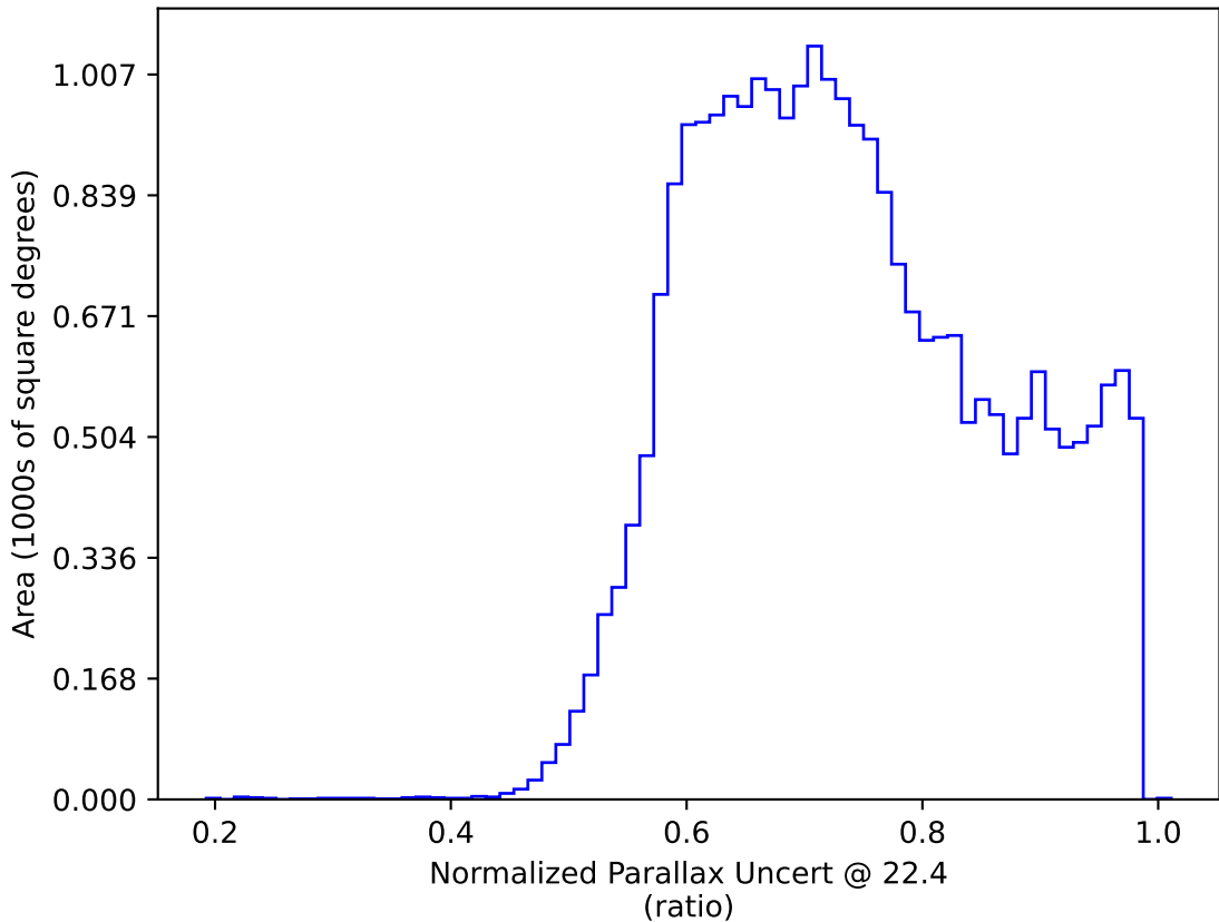
ddf_loaded_half_fl2_v3.4_10yrs All sky: Normalized Parallax Uncert @ 22.4
